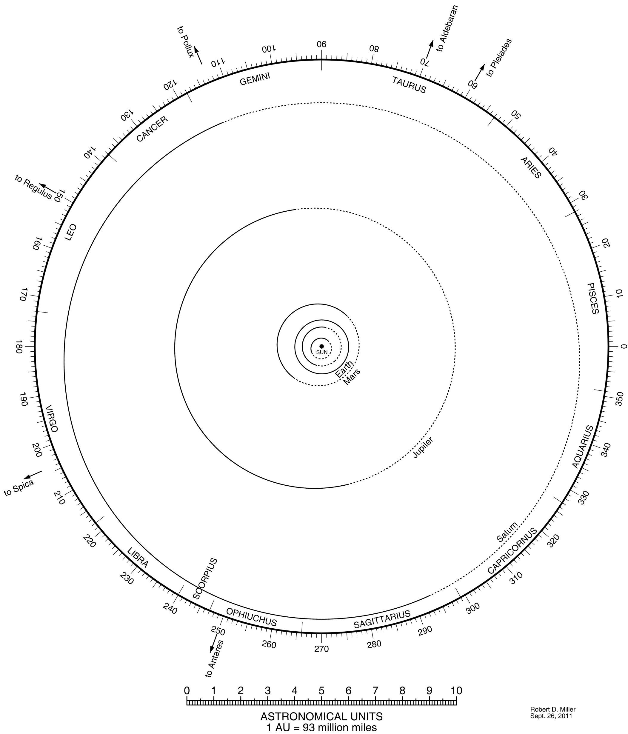
Chart of Planetary Orbits Mercury through Saturn
